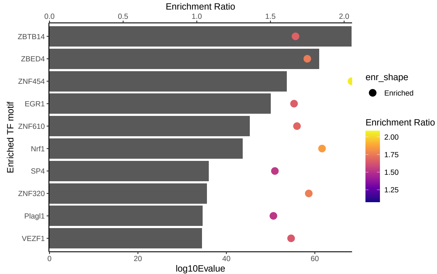
filtered_H3K9me3_Set3_data - 10
